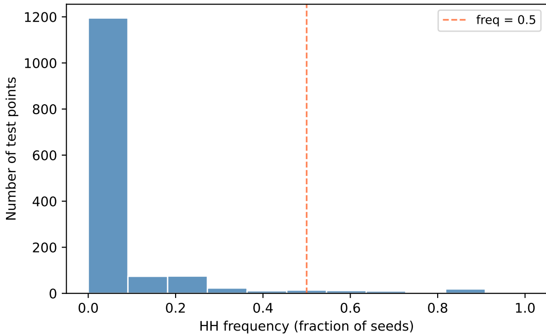
HH selection frequency histogram — compas
