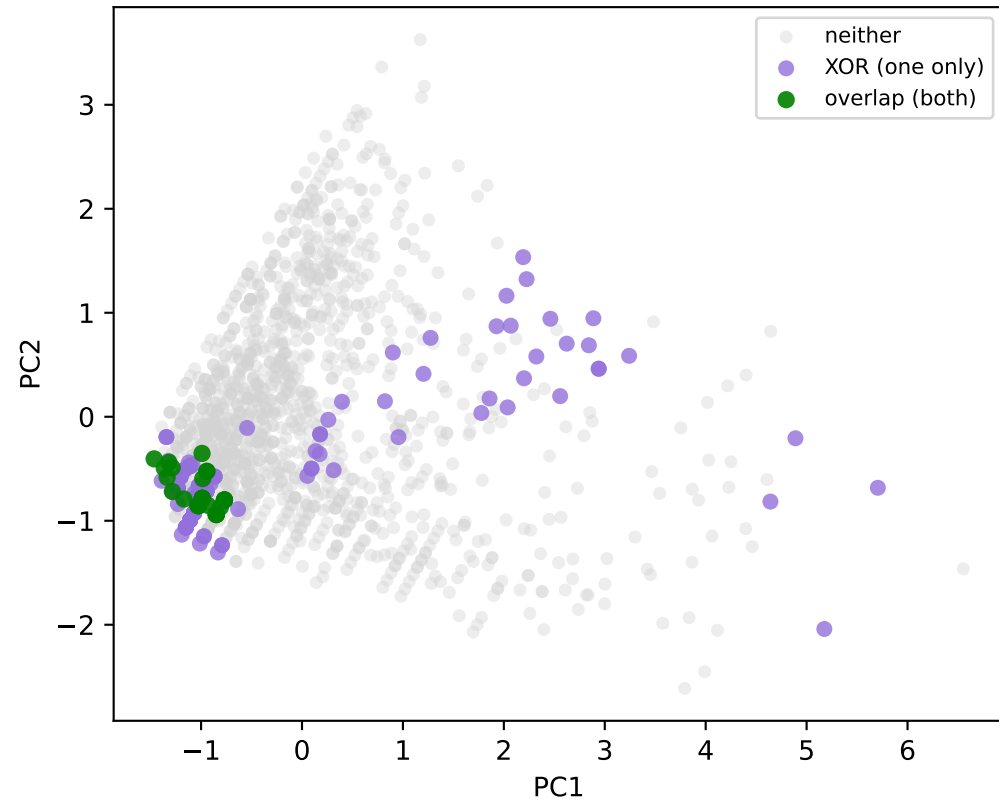
Overlap vs Symmetric Difference
