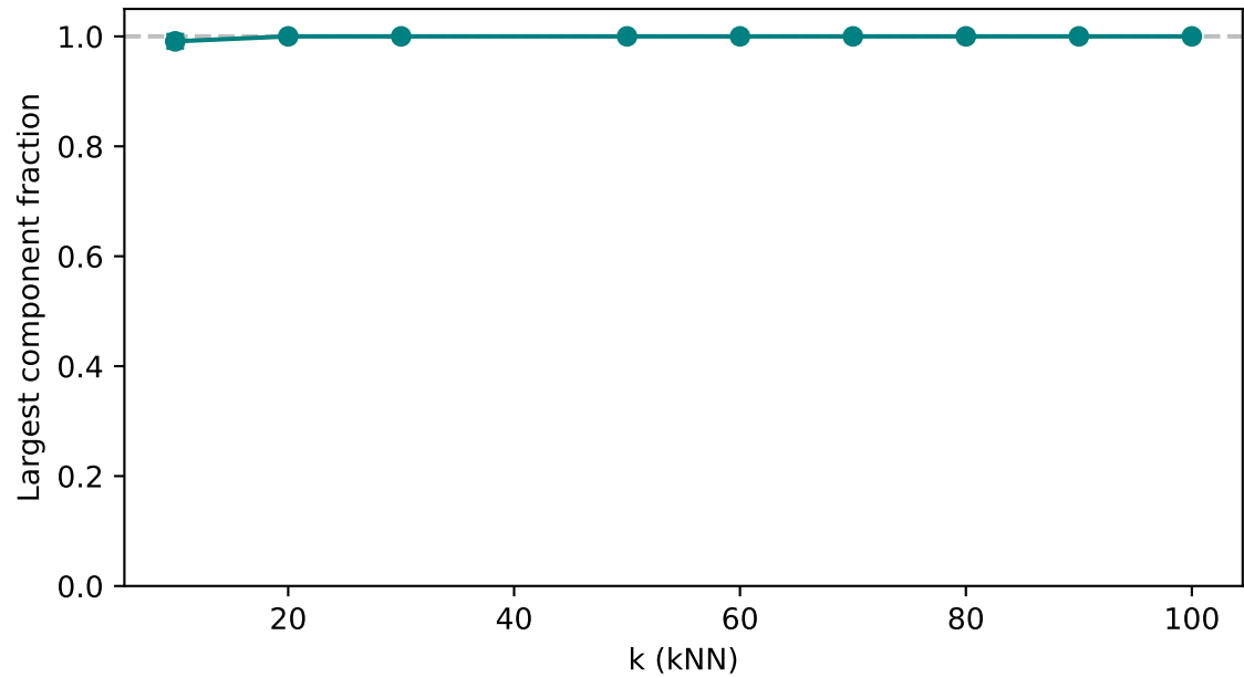
Largest component — compas
