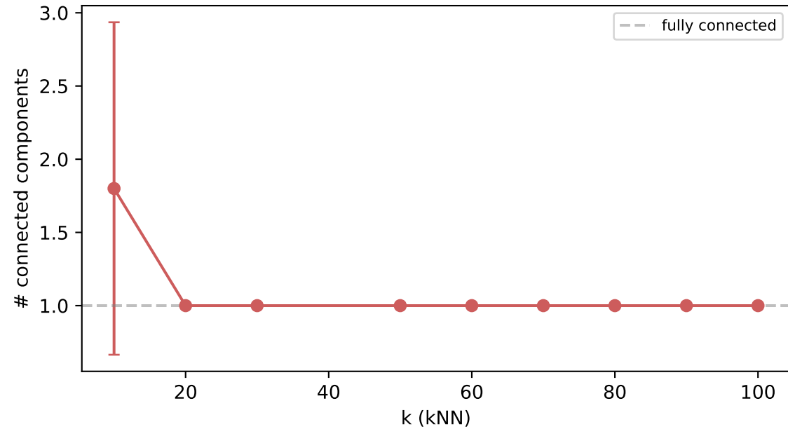
Components vs k — compas
