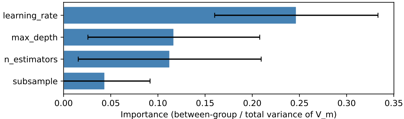
adult — GBM: top HP importance (mean \pm std over seeds)
