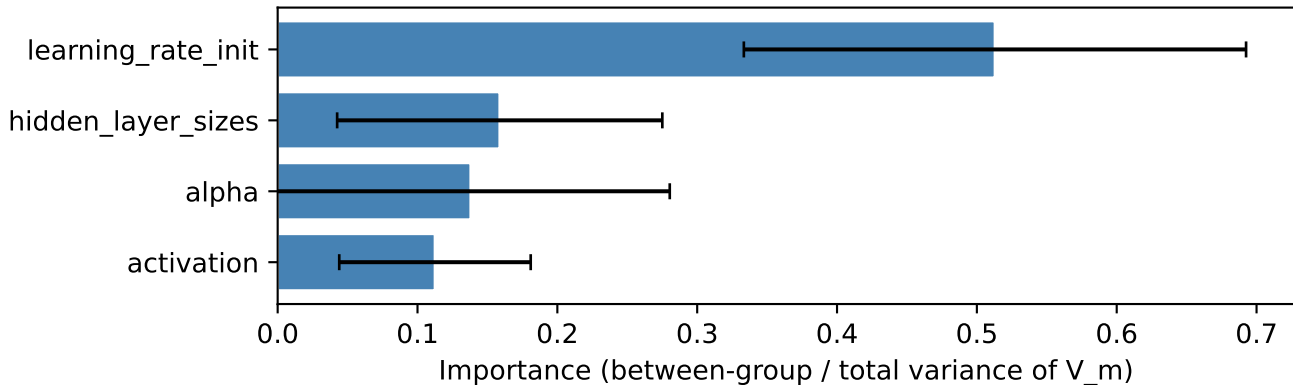
adult — MLP: top HP importance (mean \pm std over seeds)
