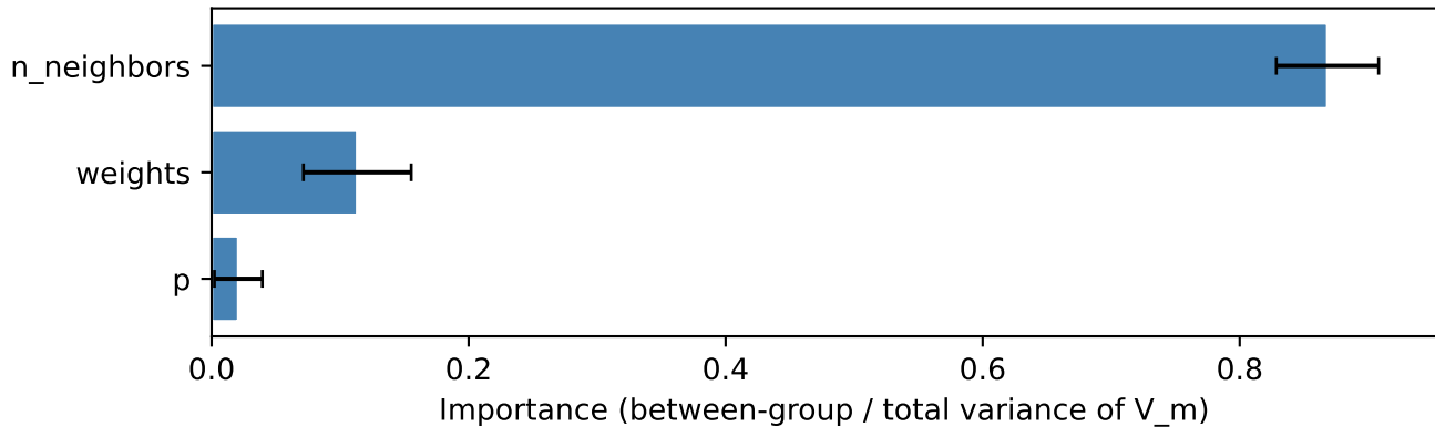
adult — kNN: top HP importance (mean \pm std over seeds)
