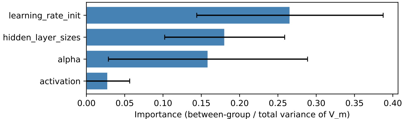
compas — MLP: top HP importance (mean \pm std over seeds)
