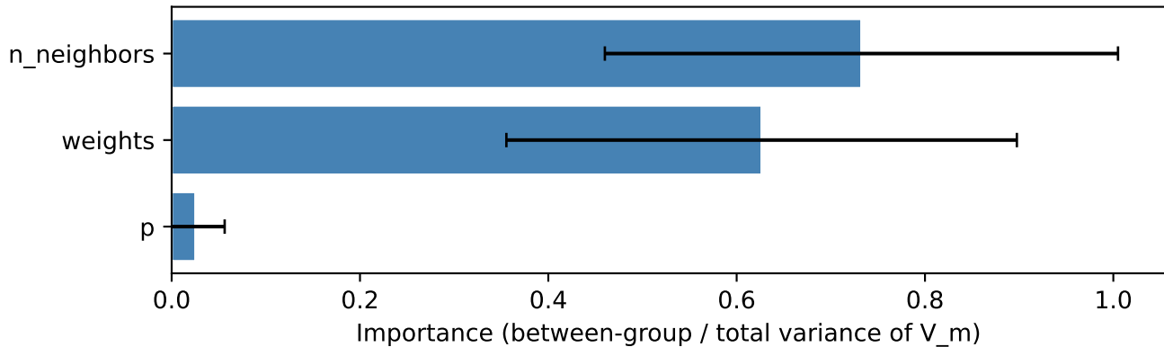
compas — kNN: top HP importance (mean \pm std over seeds)
