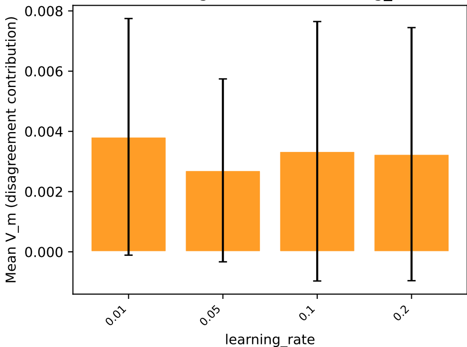
adult — GBM: marginal effect of learning_rate on V_m
