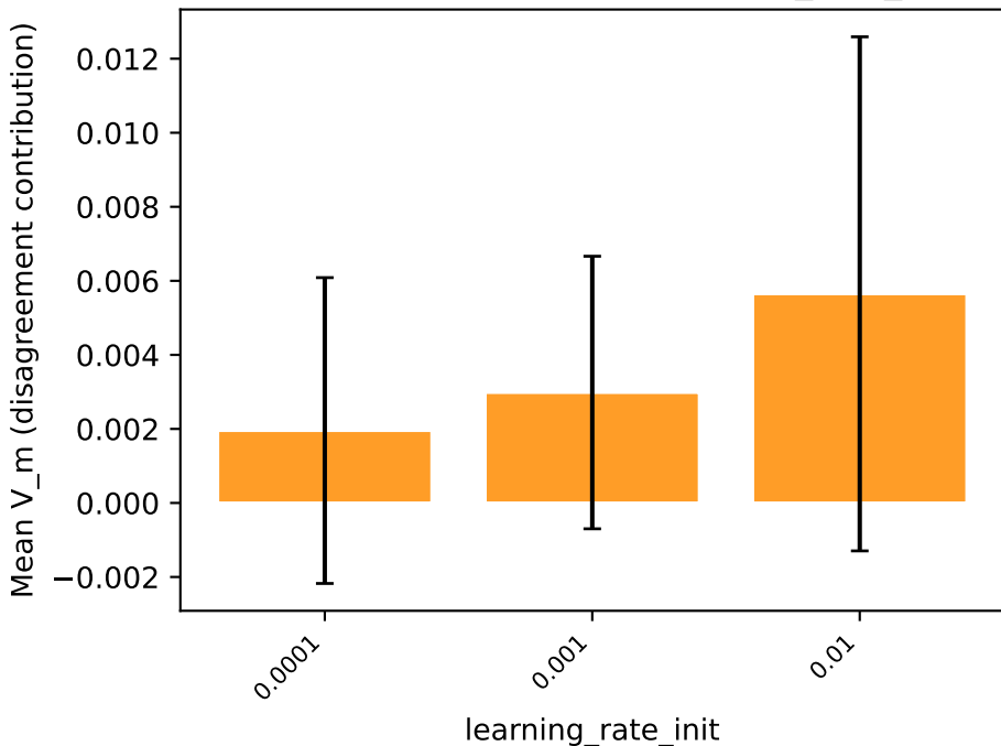
adult — MLP: marginal effect of learning_rate_init on V_m
