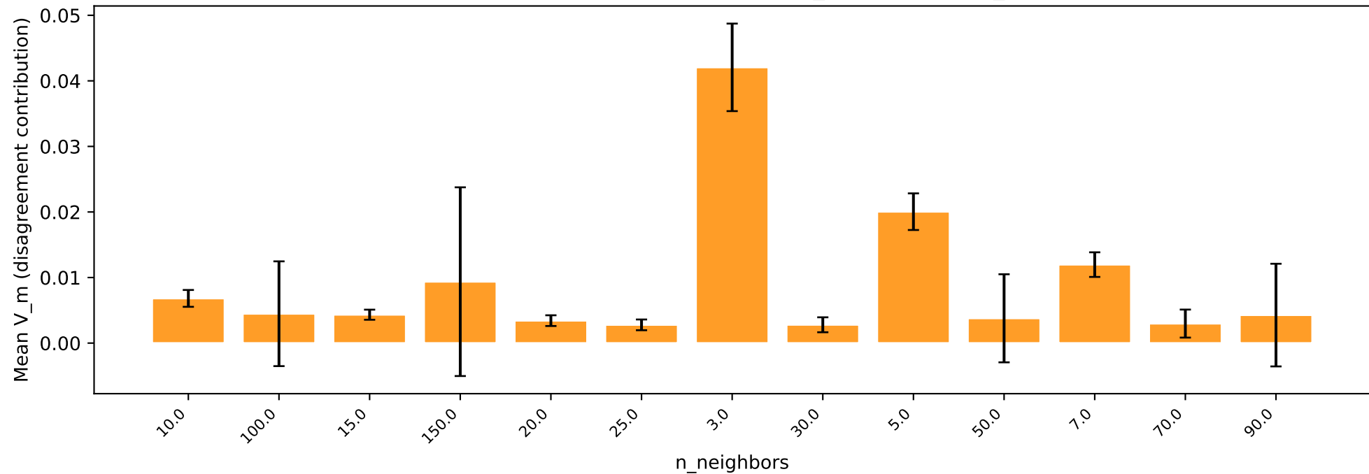
adult — kNN: marginal effect of n_neighbors on V_m
