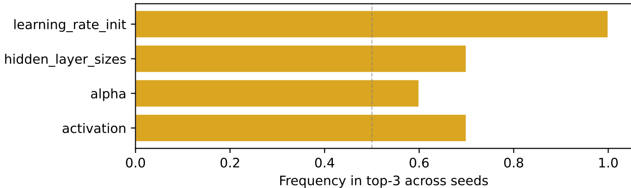
adult — MLP: rank stability (top-3 frequency)
