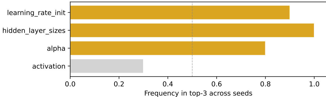
compas — MLP: rank stability (top-3 frequency)
