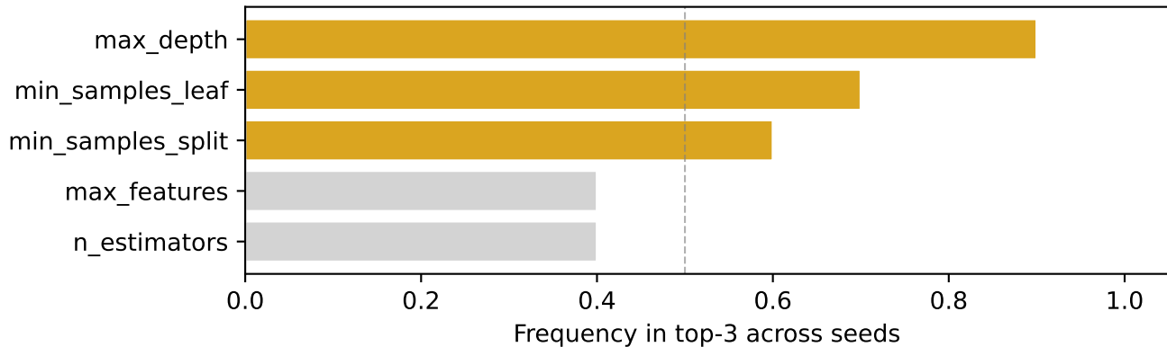
compas — RF: rank stability (top-3 frequency)
