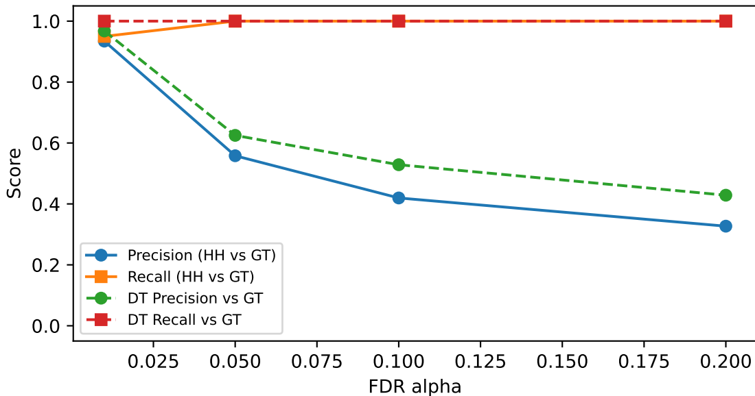
Precision & Recall vs alpha (structural exceptions)
