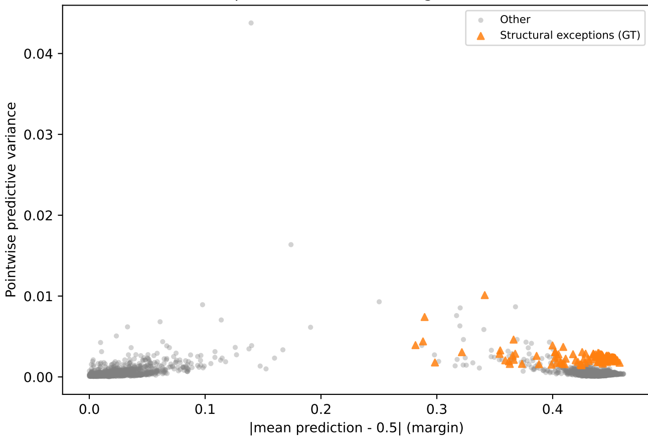
Structural exceptions: variance vs margin (Pearson r=0.018 )
