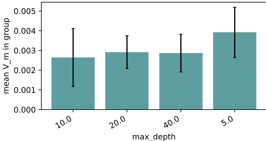
compas — RF: marginal V_m by max_depth
