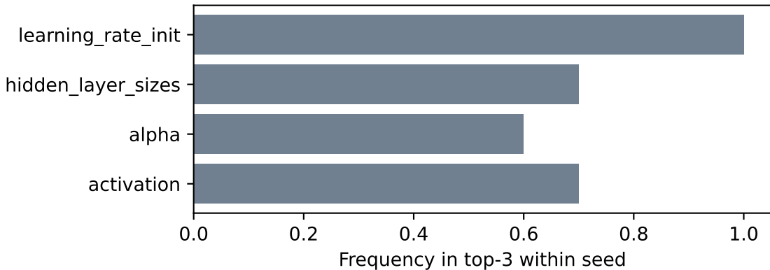
adult — MLP: rank stability (V_m importance)
