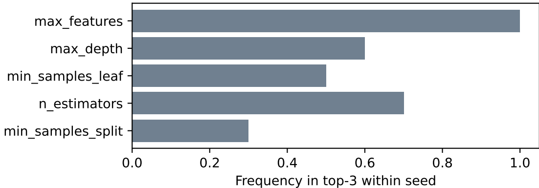
adult — RF: rank stability (V_m importance)
