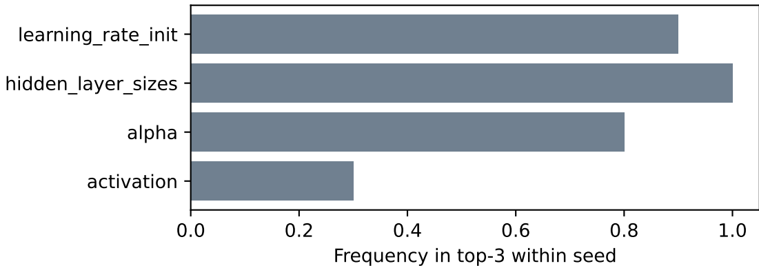
compas — MLP: rank stability (V_m importance)
