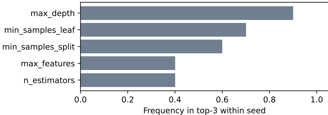
compas — RF: rank stability (V_m importance)
