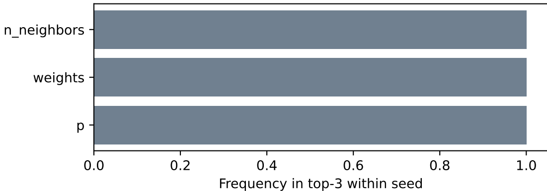
compas — kNN: rank stability (V_m importance)
