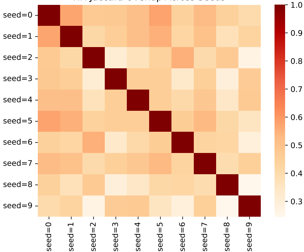
HH Jaccard Overlap Across Seeds
