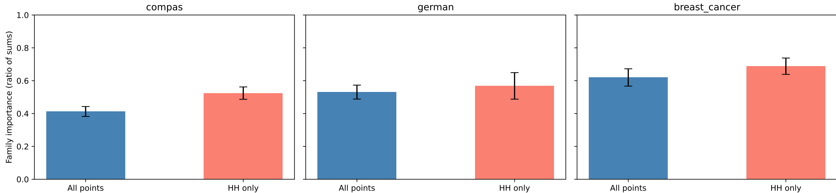
Family importance: All vs HH (mean \pm std across seeds)
