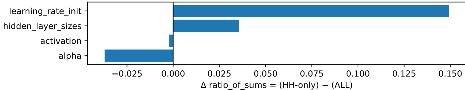
compas | seed=0 — MLP: hotspot-specific HP drivers
