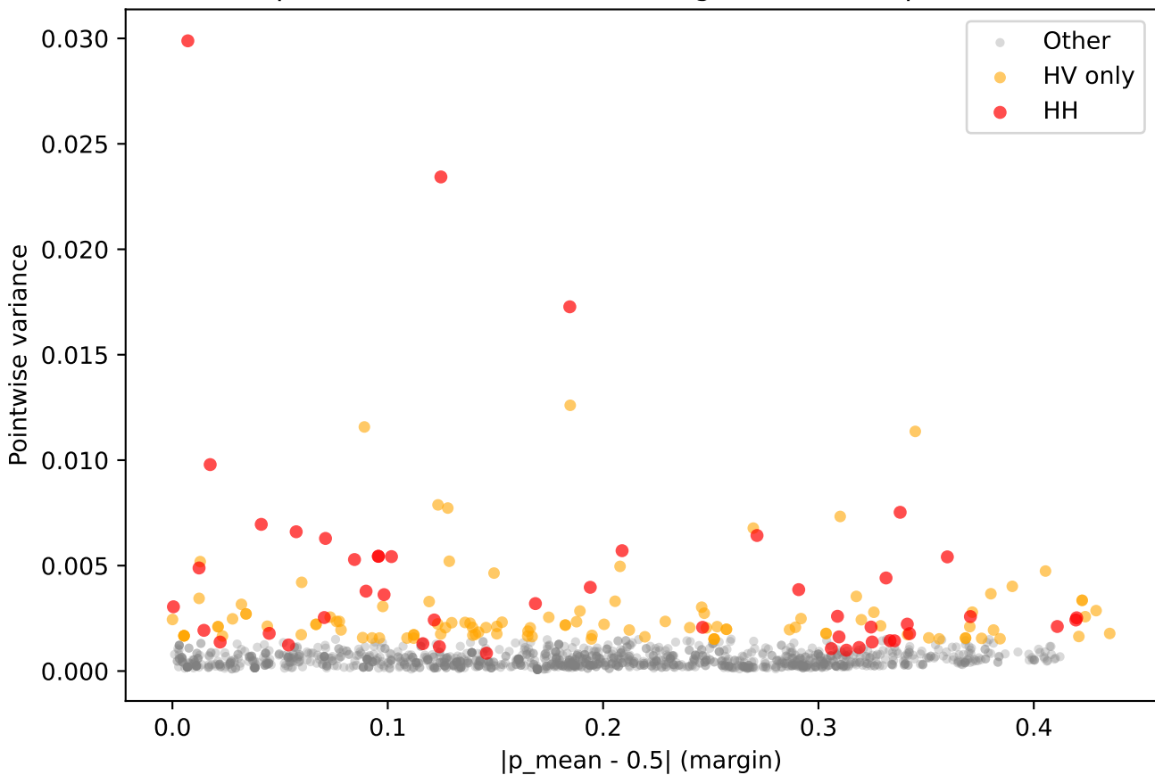
compas seed=0: variance vs margin ( r=-0.019 , p=4.8e-01 )
