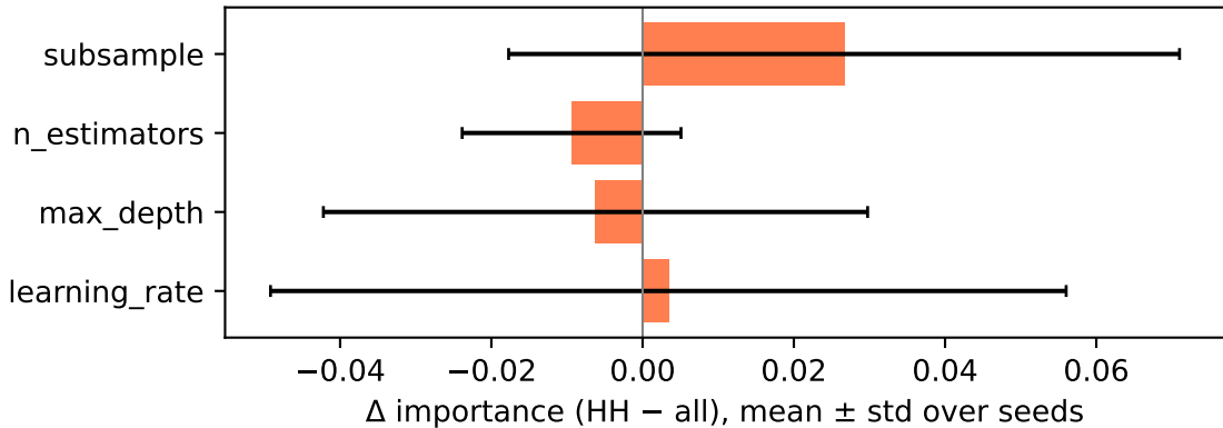
compas — GBM
