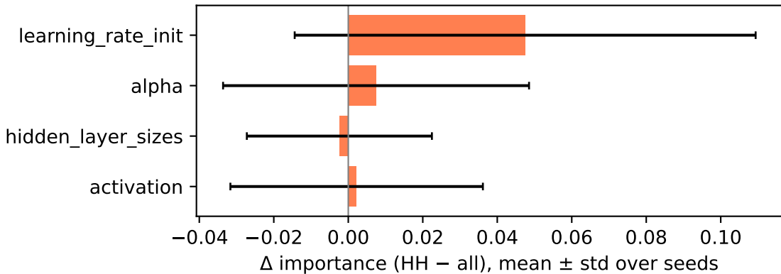
compas — MLP
