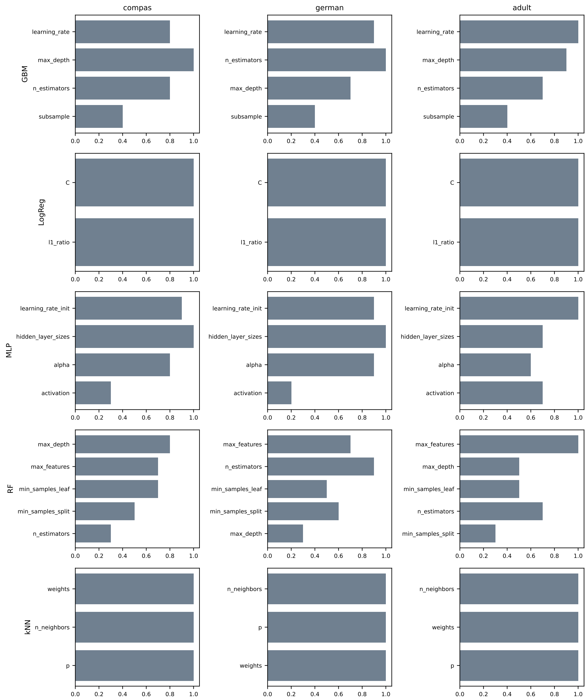
Secondary: top-3 rank frequency ( V_m -by-HP-value, subset=all, Rashomon)
