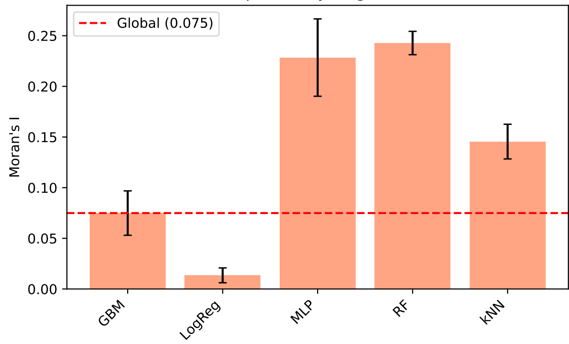
Moran's I: per-family vs global — Adult
