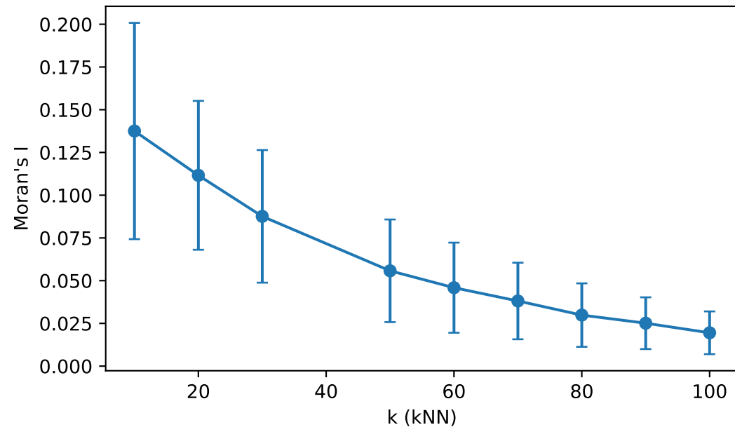
Moran's I vs k
