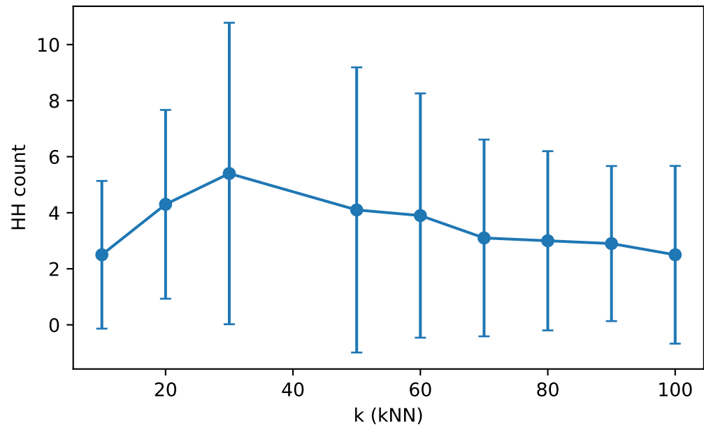
Variance-HH count vs k
