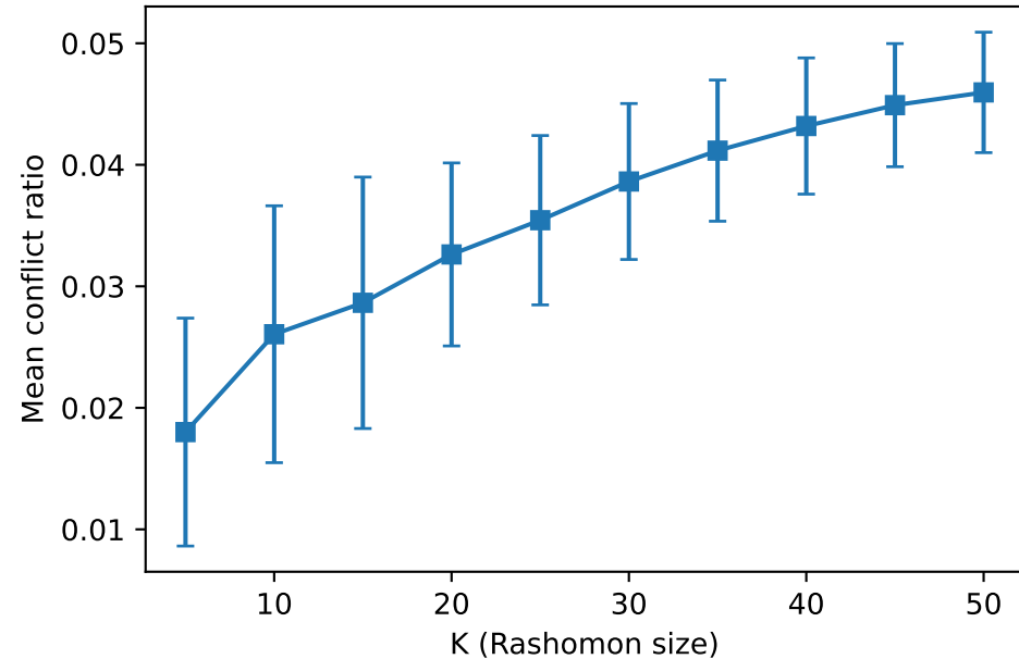
Mean conflict vs K
