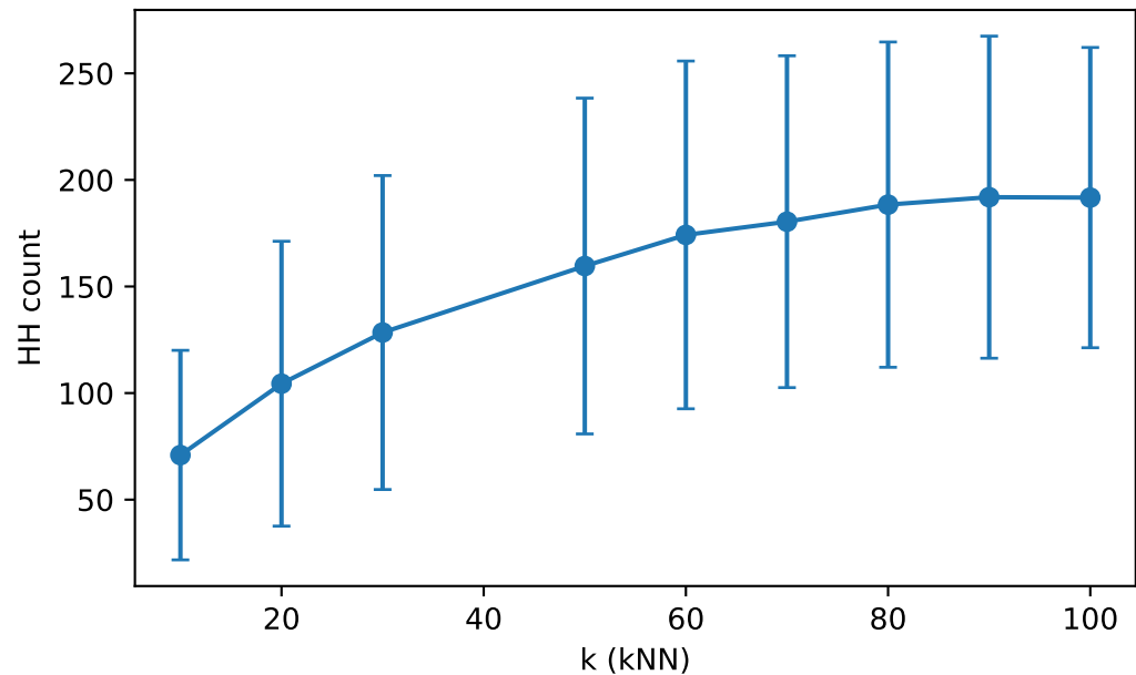
Variance-HH count vs k
