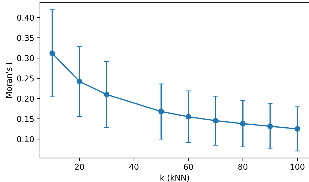
Moran's I vs k
