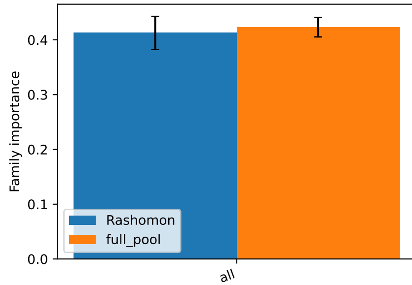
COMPAS
