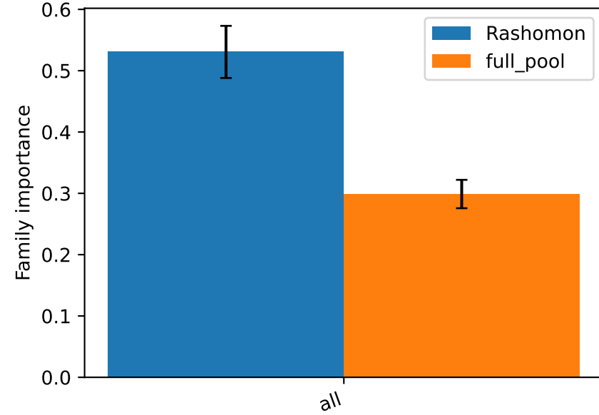
German Credit
