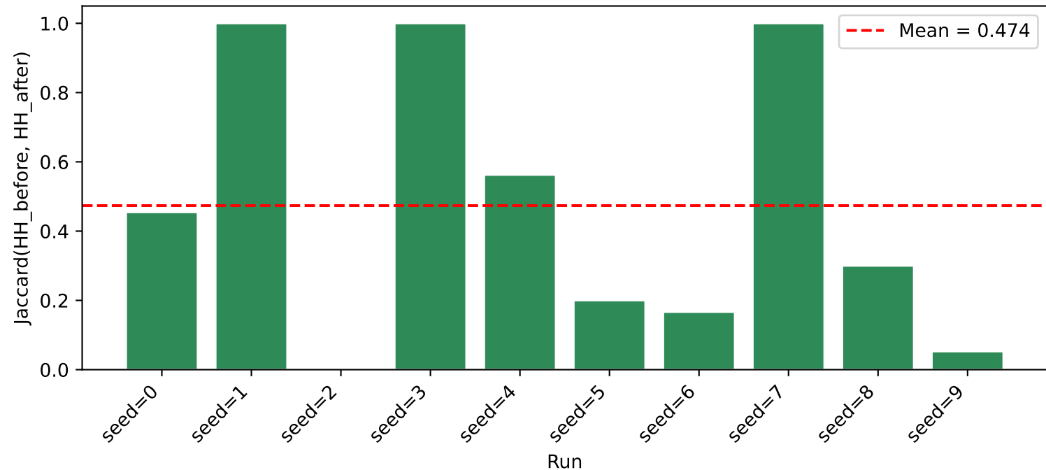
HH mask overlap: before vs after — German Credit (platt)
