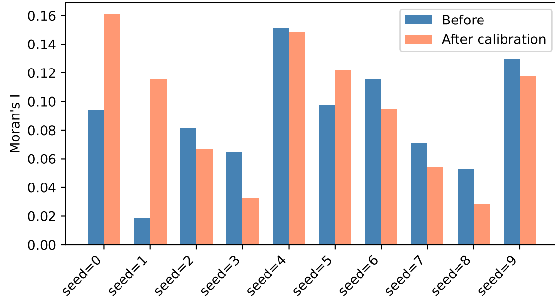
Moran's I: before vs after — German Credit (isotonic)
