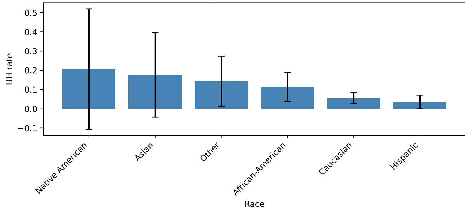
COMPAS: HH rate by race (mean \hat{A} \pm std across 10 seeds)
