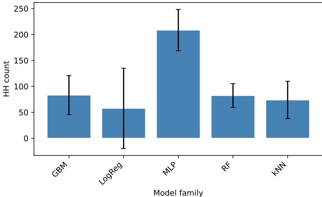
HH count by family (Compas, per-family top-25, mean \pm std over runs)
