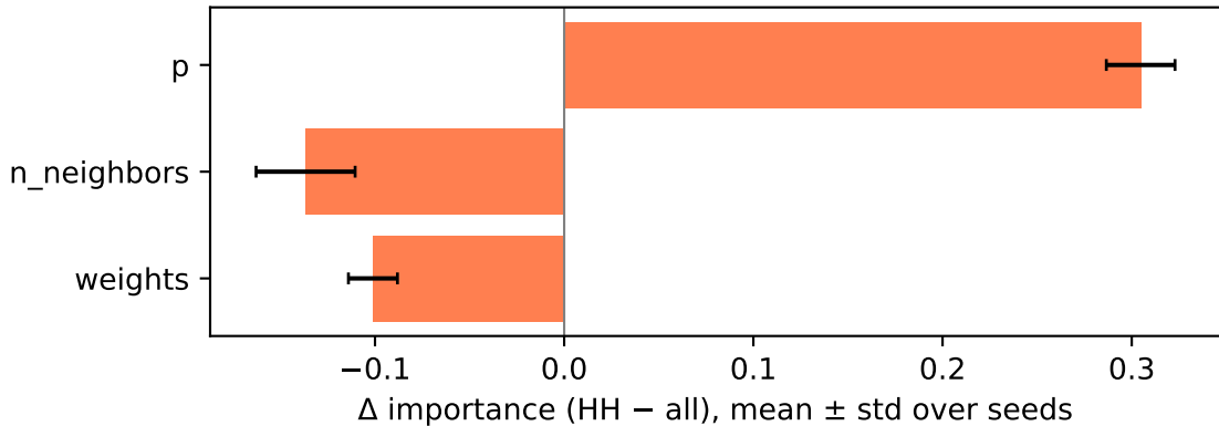
adult — kNN
