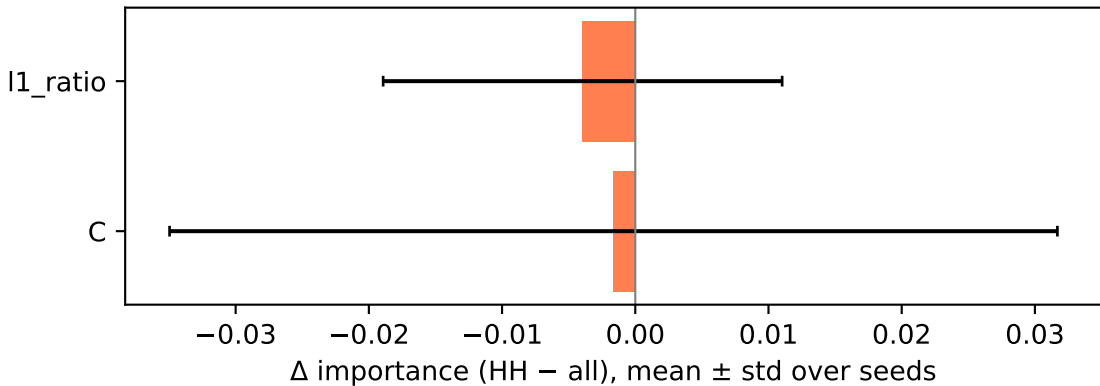
compas — LogReg
