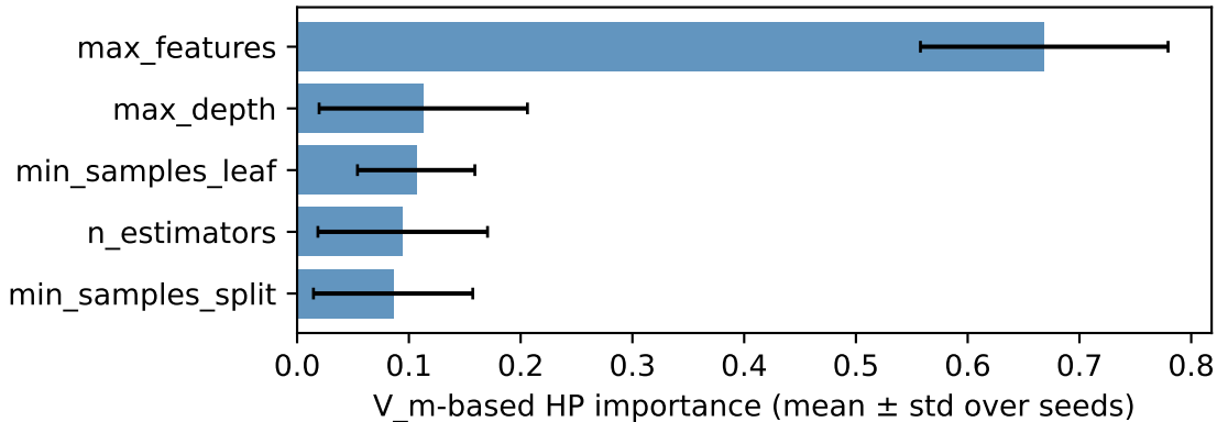
adult — RF — subset=all
