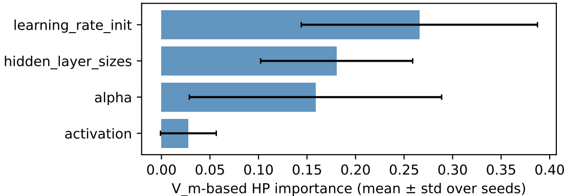
compas — MLP — subset=all
