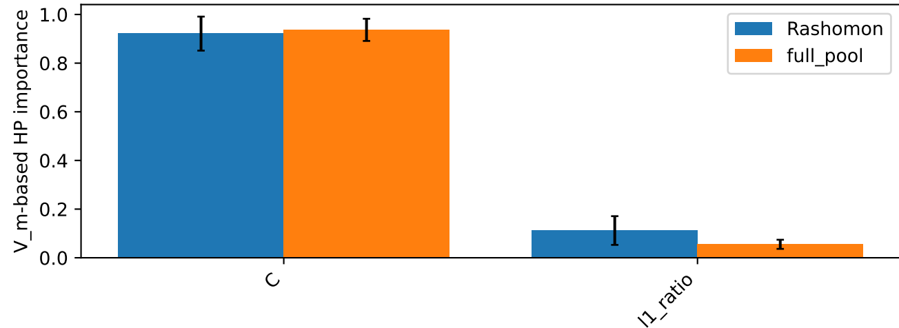
adult — LogReg — subset=all
