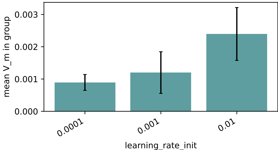
adult — MLP: marginal V_m by learning_rate_init
