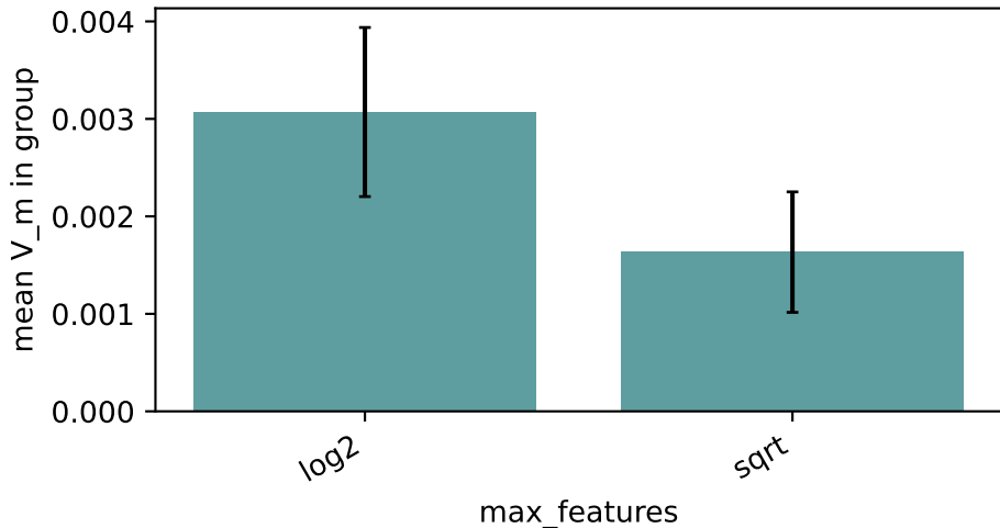
adult — RF: marginal V_m by max_features
