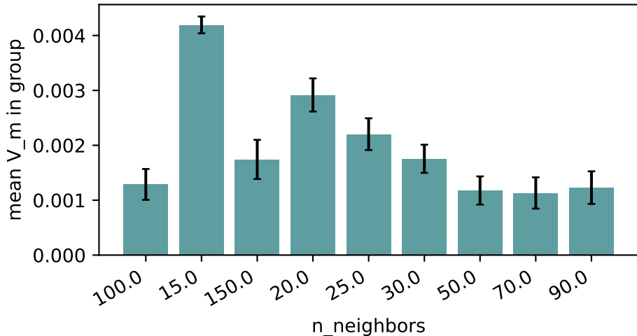
adult — kNN: marginal V_m by n\_neighbors
