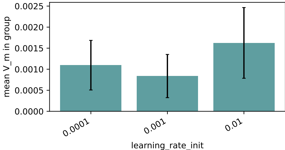
compas — MLP: marginal V_m by learning_rate_init
