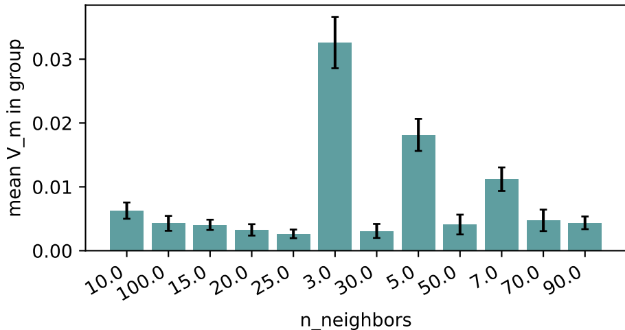
german — kNN: marginal V_m by n\_neighbors
