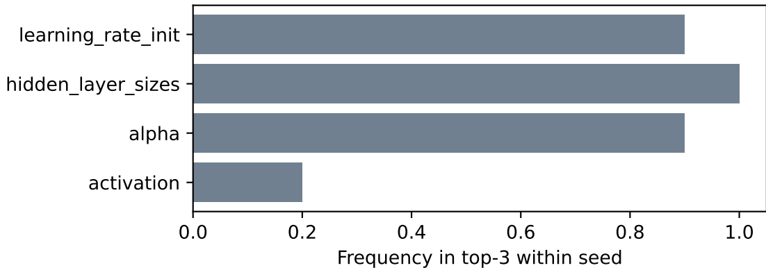
german — MLP: rank stability (V_m importance, subset=all)
