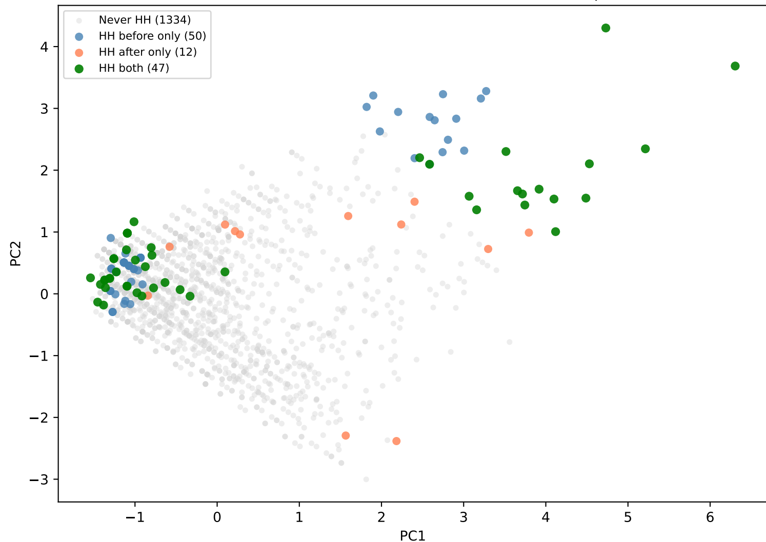
HH movement: before vs after isotonic calibration — compas (seed=6)
